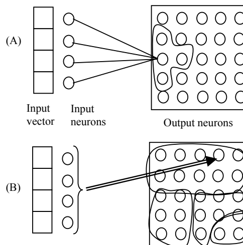
Figure 1 – Self-organizing Classification
