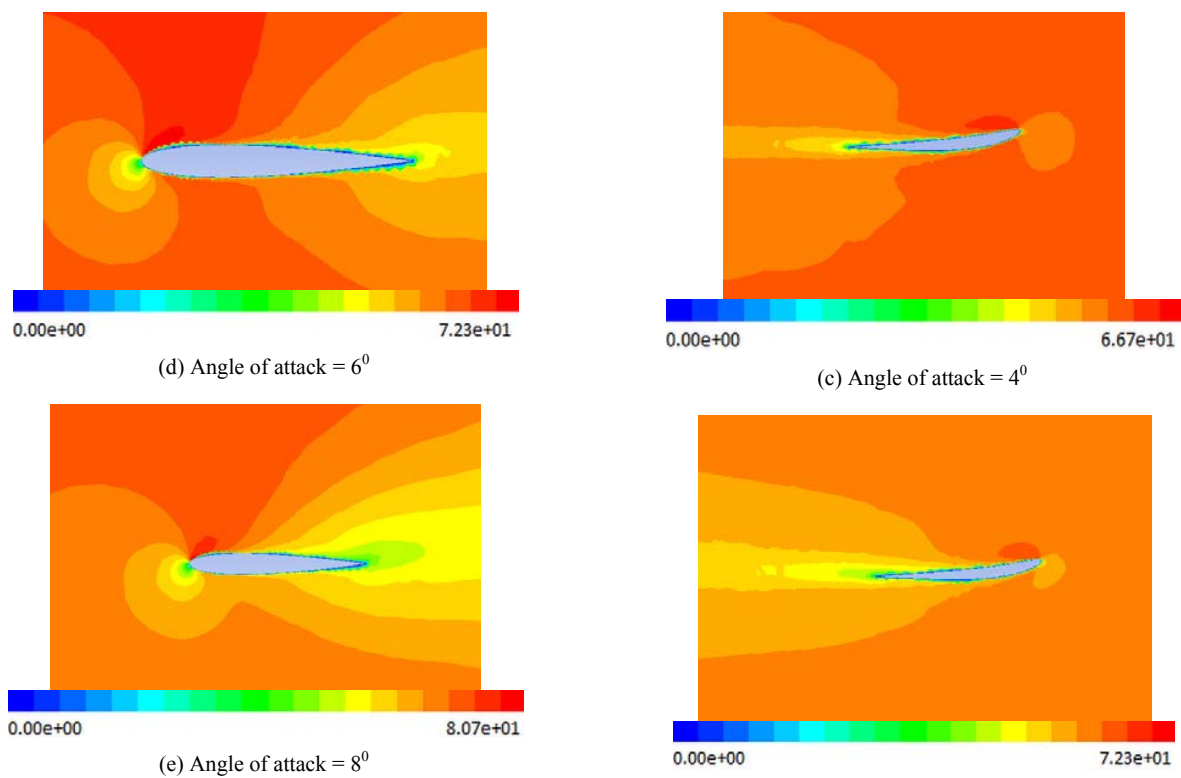
Fig. 14 (a)-(e) Velocity contours (meters per second) at cant angle 15^\circ at symmetry plane with different angles of attack
