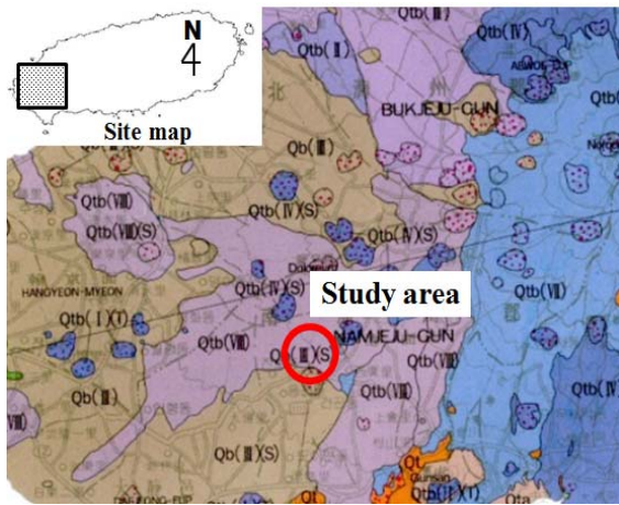
Fig. 1 Geologic map of study area
