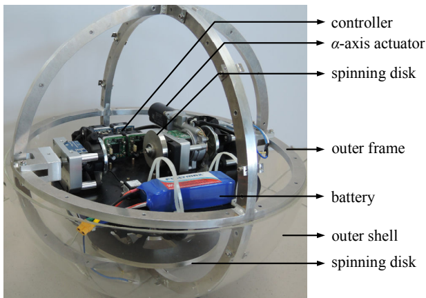
Fig. 8 The preliminary prototype of the 3DF robot
