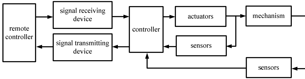
Fig. 2 The scheme of the control system
