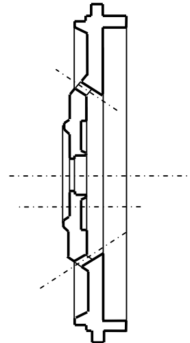
Fig. 19 A sketch of a Flywheel
