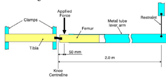
Fig. 7 Top view of test setup for static legform impactor shearing certification [2]
