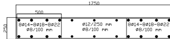
Fig. 3 Cross section of rectangular shear walls
