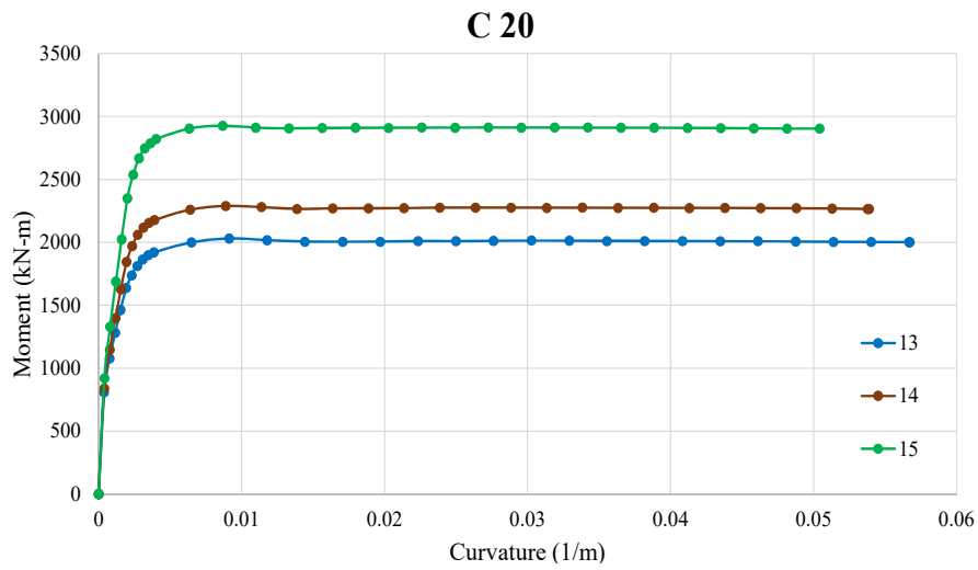
Fig. 7 (a) MC relationship with longitudinal reinforcement type
