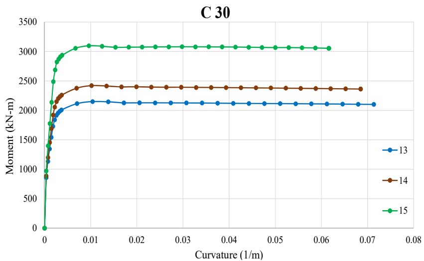
Fig. 7 (b) MC relationship with longitudinal reinforcement type
