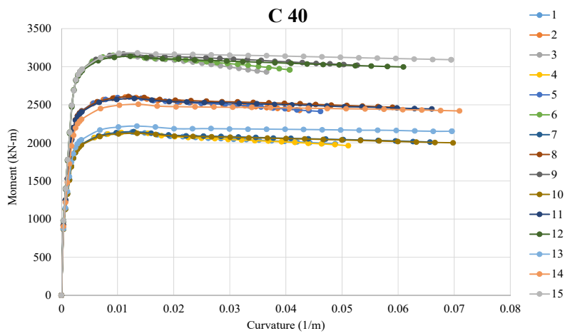
Fig. 5 (c) MC relationship for C40
