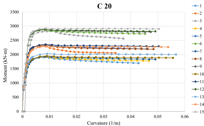
Fig. 5 (a) MC relationship for C20
