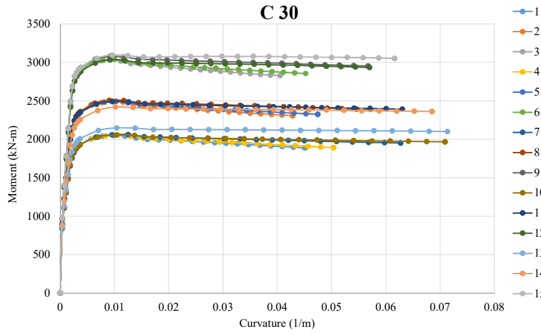
Fig. 5 (b) MC relationship for C30
