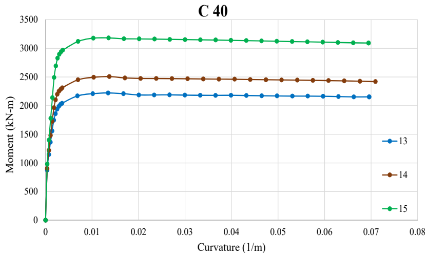
Fig. 7 (c) MC relationship with longitudinal reinforcement type
