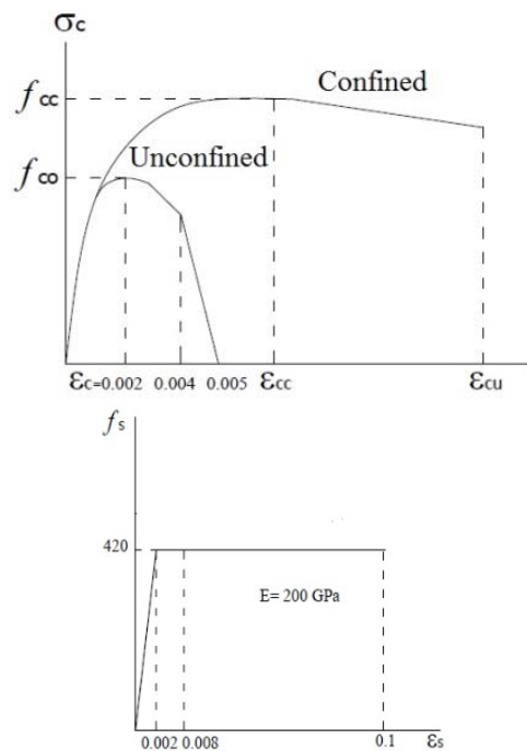
Fig. 4 Stress-strain relationship for materials
