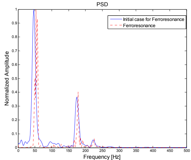
Fig. 8 Comparisons of the PSDs for ferroresonance regions
