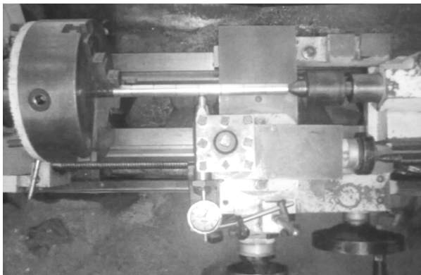
Fig. 2 Experimental setup for burnishing process on Lathe machine
