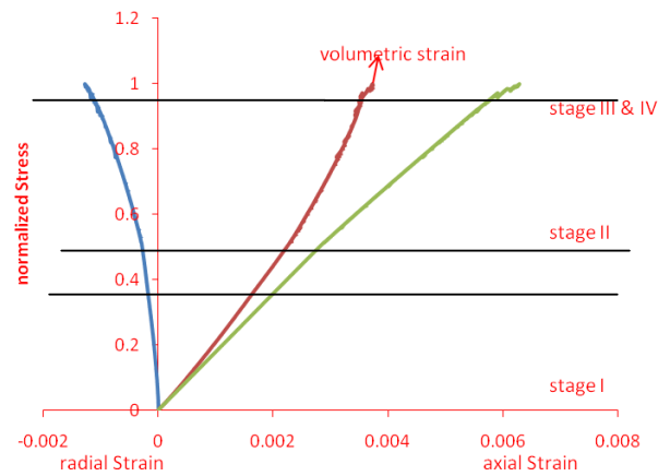
Fig. 13 Normalised stress-strain curves, Quartzite2 specimen
