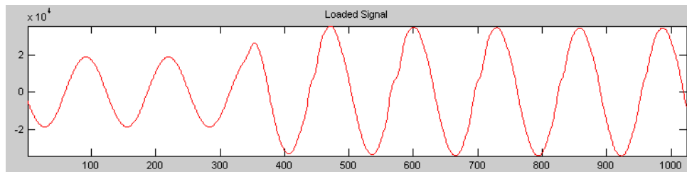
Fig. 2 Voltage swell
