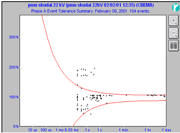
Fig. 7 CBEMA curve
