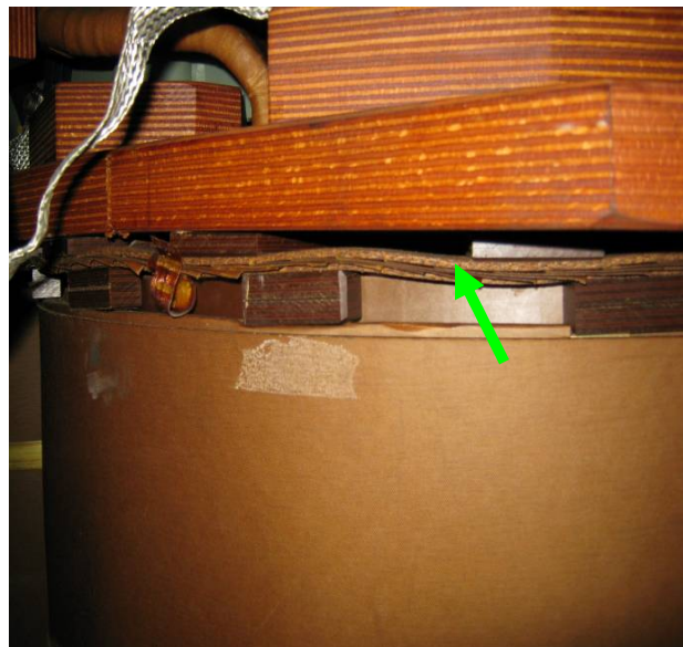
Fig. 8(a): Wavy pressboard due to coaxial force
