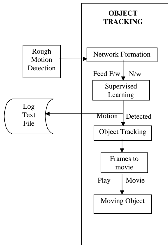
Fig. 6 Object Tracking
