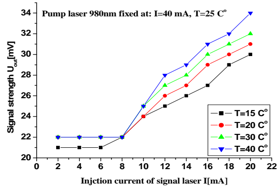
Fig. 3 Signal strength in mV versus the injection current in mA of signal laser 1550 nm by fixed I= 40 mA ant T=25 C° of pump laser 980nm
