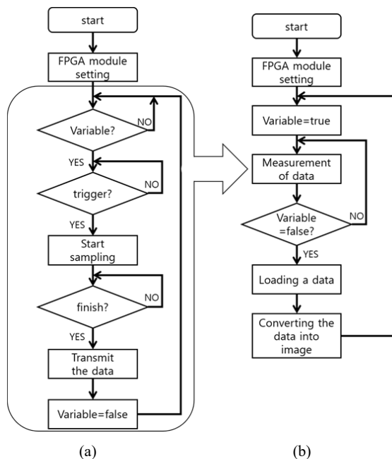
Fig. 2 Program flow chart (a) FPGA (b) Host
