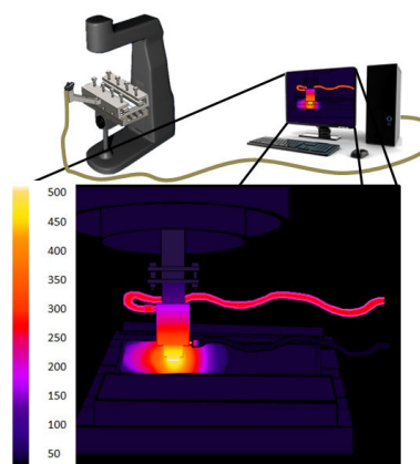
Fig. 7 Simulated thermographic image during FSW
