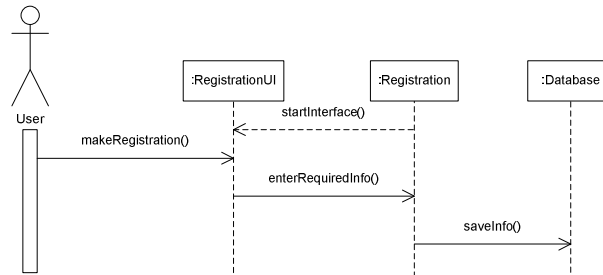
Fig. 6 Sequence diagram for registration
