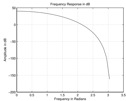
Fig. 3. Frequency Response in dB of H(z) of Equation (15)
