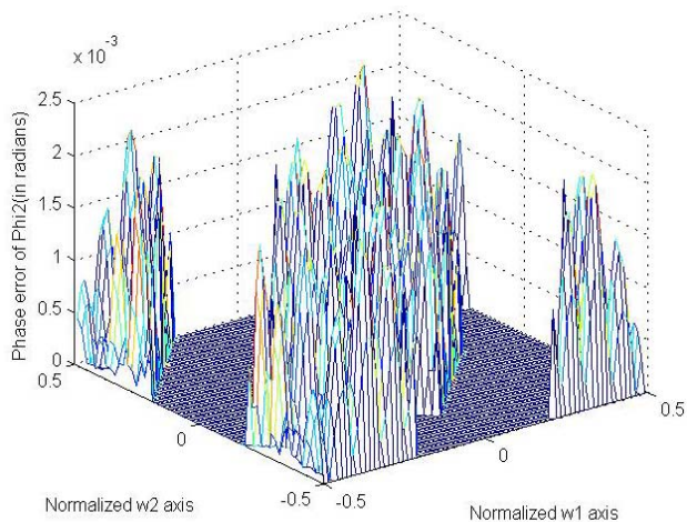
Fig. 8 Phase response error of the denominator of A_2(e^{j\omega_1}, e^{j\omega_2})
