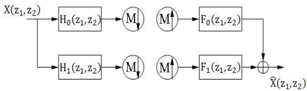
Fig. 2 The structure of conventional 2-D QMF banks
