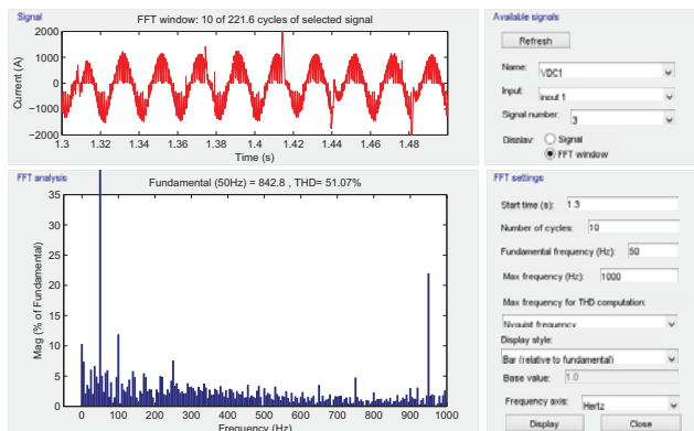
Fig. 18. The steady state current source and FFT analysis of the RTS output
