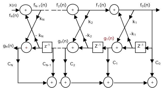
Fig.1 Structure of Lattice-ladder IIR filter oh N^{th} order
