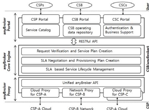
Fig. 1 anyBroker whole architecture
