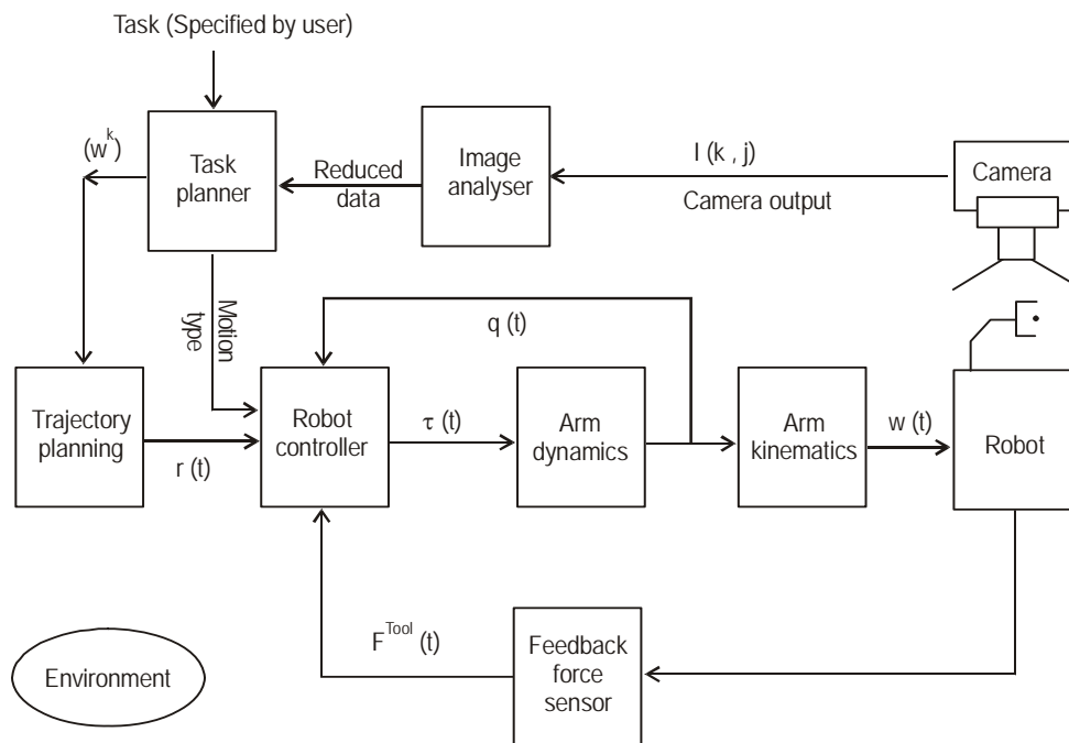
Fig. 4 A rudimentary task planner
