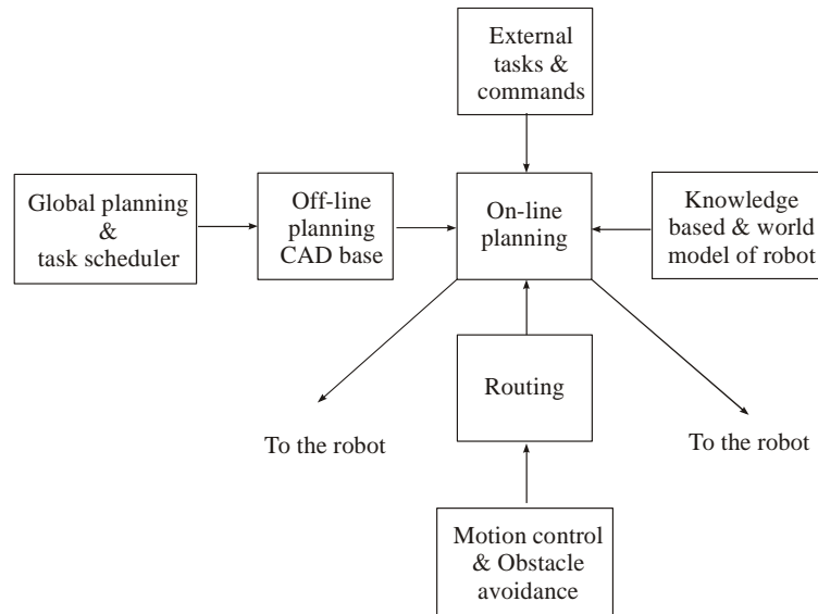
Fig. 5 Task planner design algorithm for stationary &amp; mobile robots
