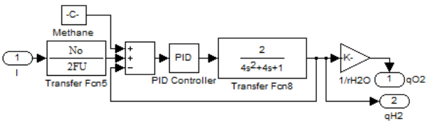
Fig. 7 Reformer model
