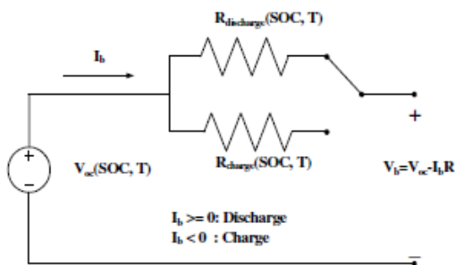
Fig. 4 Battery model
