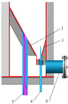
Fig. 4 Grid with tangential injection of the fluidizing gas into the chamber
