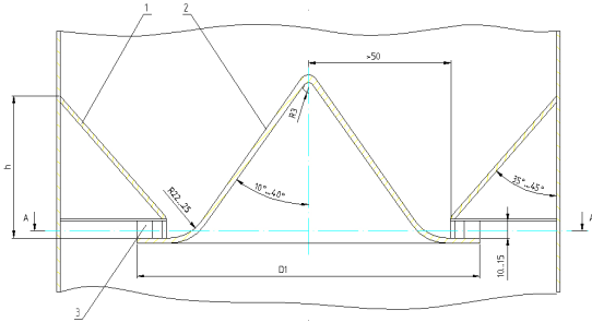
Fig. 10 Constructive design of the grid
