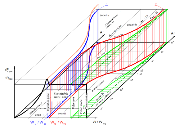
Fig. 9 Working regions of fluidized systems
