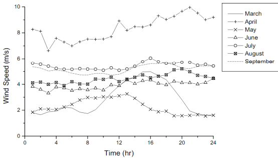
Fig. 1 Average wind speed at Sandwip in March–September
