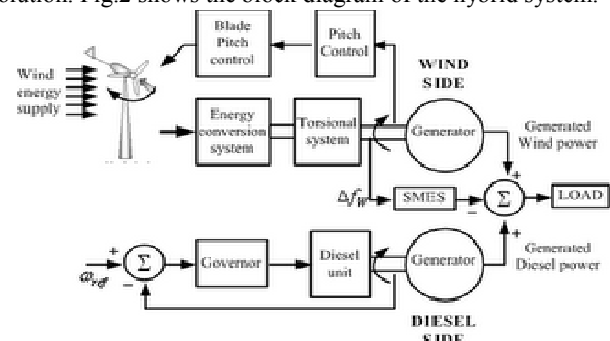
Fig. 2 Block diagram of wind-diesel hybrid power system
