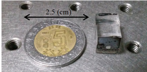
Fig. 5 Fabricated Herriott cell integrated on an acrylic slab with d = 1.5 cm and R = 3 cm
