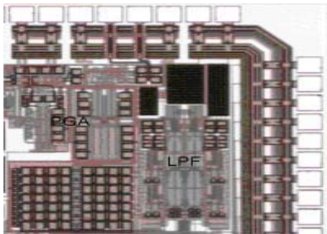
Fig. 8 Chip photograph
