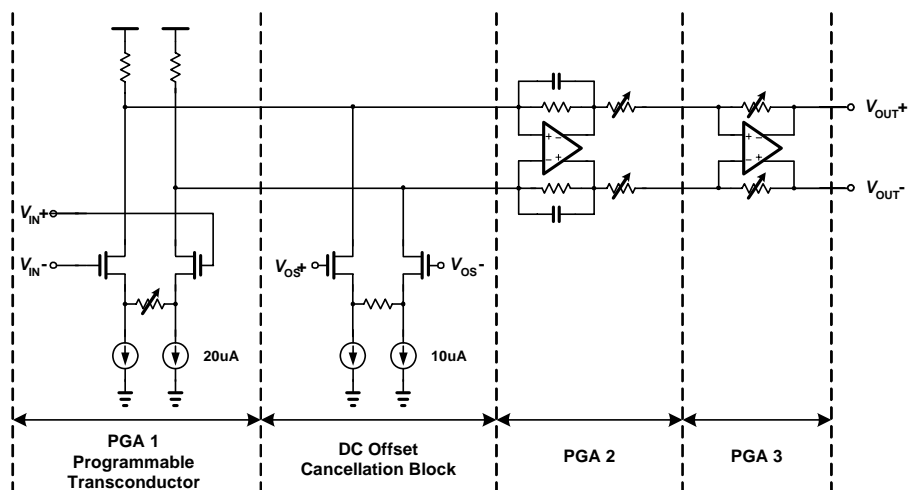
Fig. 4 Circuit schematic of the PGA
