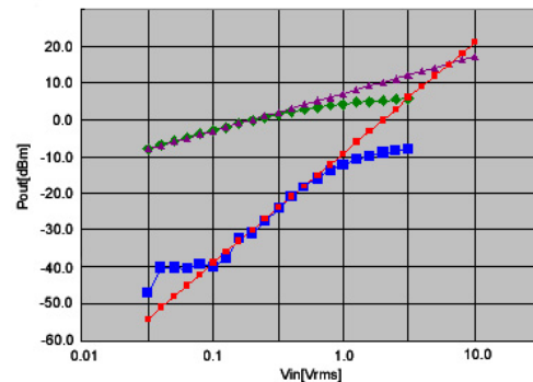
Fig. 9 The third-order intercept point of the AFE
