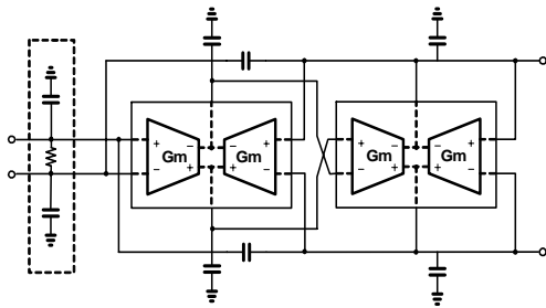
Fig. 2 The designed third order Butterworth LPF
