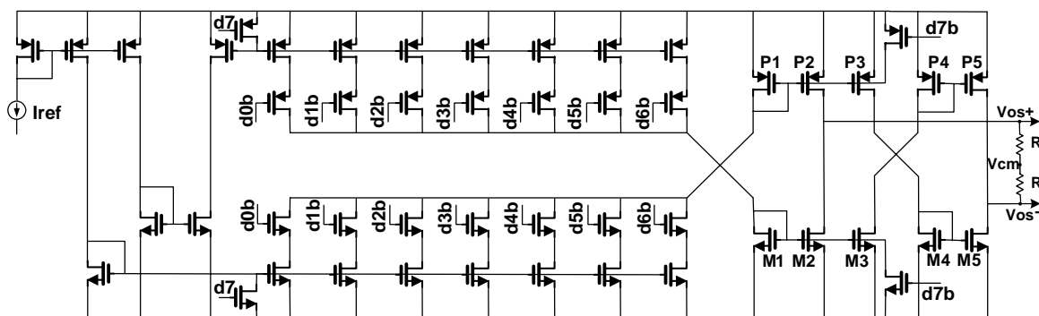
Fig. 7 DAC for DC offset adjustment
