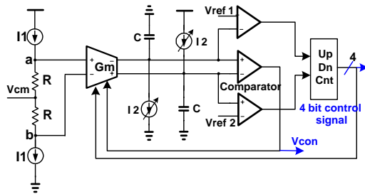
Fig. 5 Tuning Circuit
