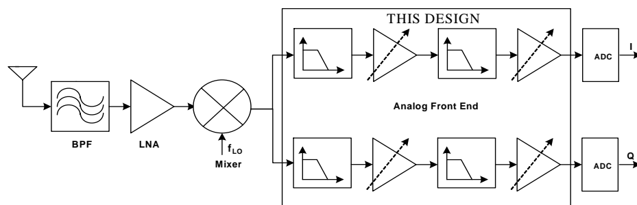
Fig. 1 Block diagram of the analog front end
