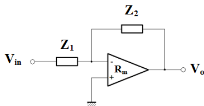
Fig. 4 Inverting amplifier
