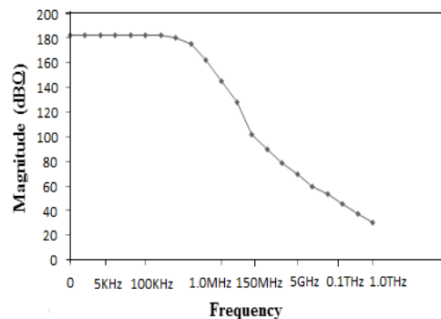
Fig. 8 Frequency characteristics of the open loop transresistance gain for the proposed circuit
