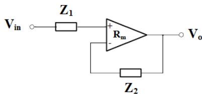
Fig. 3 Noninverting amplifier
