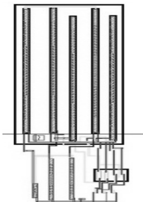
Fig. 6 Layout of the proposed differential OTRA
