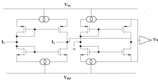
Fig. 2 Traditional circuit of an OTRA
