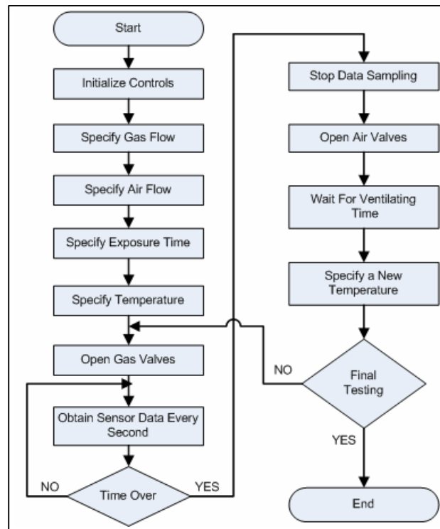
Fig.7 Interface Algorithm
