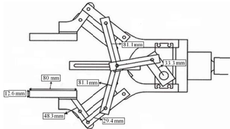
Fig. 2 Gripper model and its dimensions
