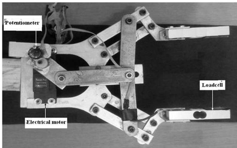
Fig. 4 Fabricated stiffness-sensitive gripper
