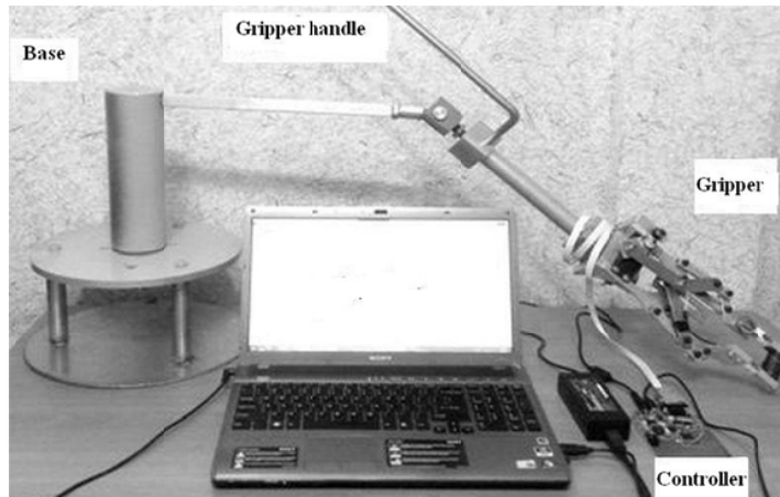
Fig. 5 Fabricated set-up for experiments
