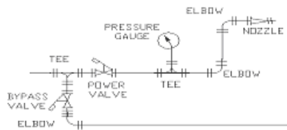
Fig. 3 Proposed pico-hydro piping system
