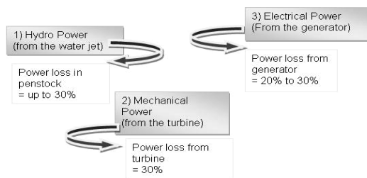
Fig. 2 Power loss during the conversion from hydro power to electricity
