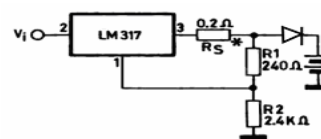
Fig. 8 Simple battery charger using LM317 voltage regulator
