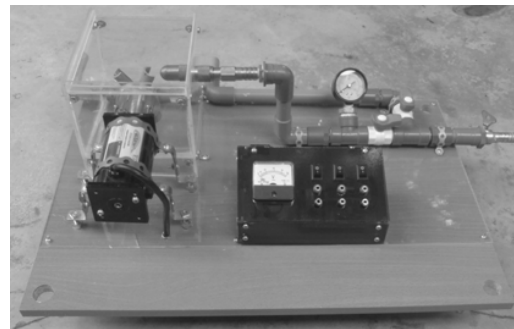
Fig. 5 Proposed pico-hydro system
