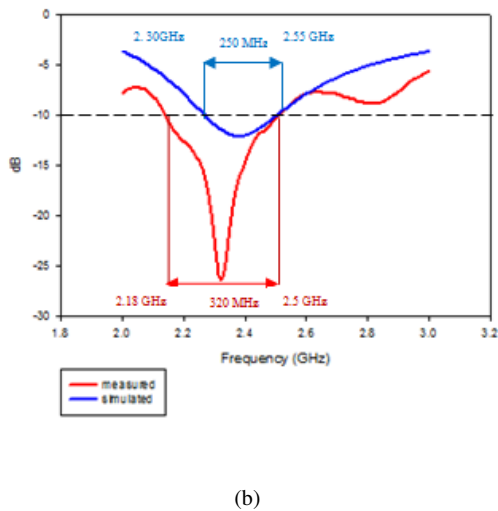
Fig. 3 Simulated and Measured S_{11} (a) BST loaded array antenna (b) BIT loaded array antenna
