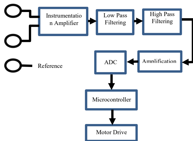
Fig. 4 Block diagram of internal circuitry
