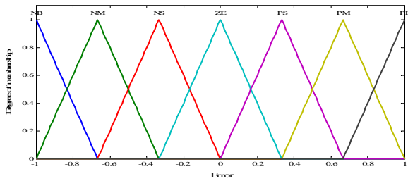
Fig. 6 Membership functions
