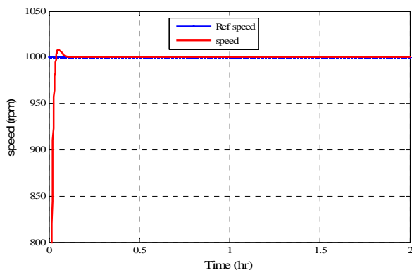
Fig. 14 Blower speed response at sudden variation
