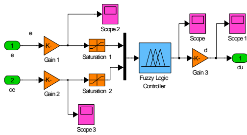
Fig. 7 AFLC architecture
