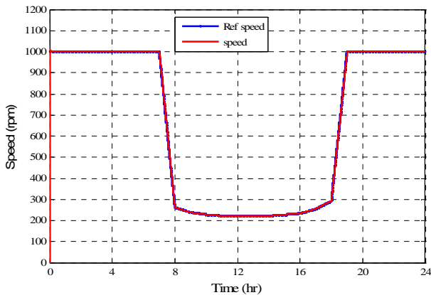
Fig. 13 Blower speed variation with reference signal
