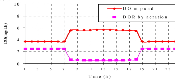
Fig. 10 Dissolved oxygen concentration
