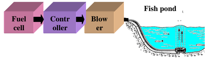
Fig. 3 Block diagram of diffused aeration
