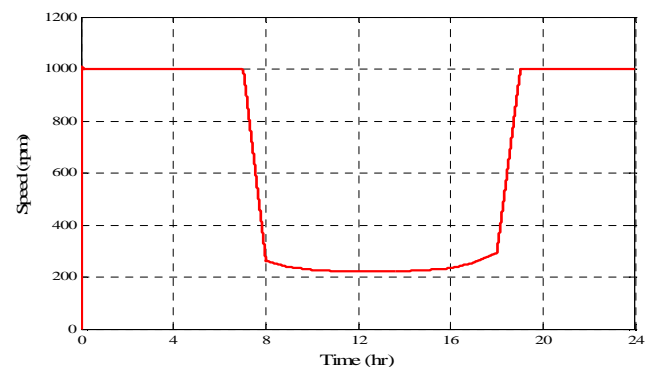
Fig. 11 Motor speed variation over the day
