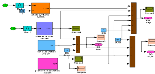
Fig. 9 Block diagram of dissolved oxygen model
