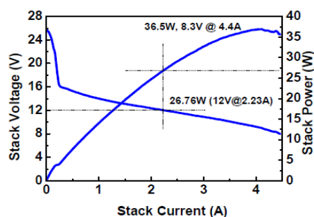
Fig. 1 Output of Fuel Cell Stacks
