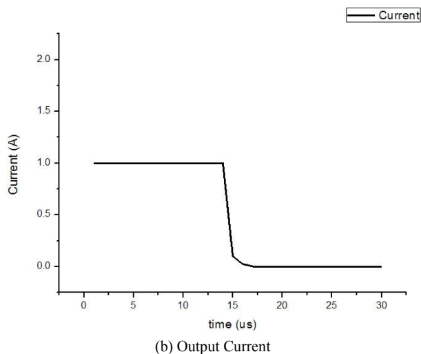
Fig. 13 Control of the Time Over-Current
