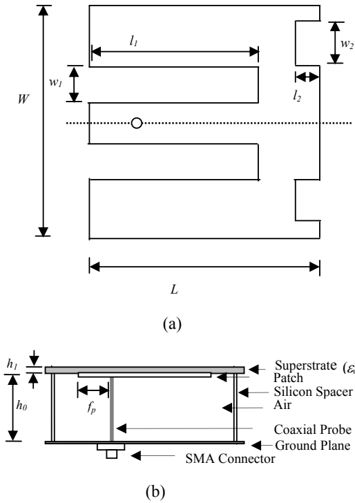
Fig.1 Geometry of proposed patch antenna. (a) Top view, (b) Side view
