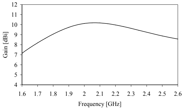
Fig. 4 Simulated gain of proposed patch antennas at different frequencies
