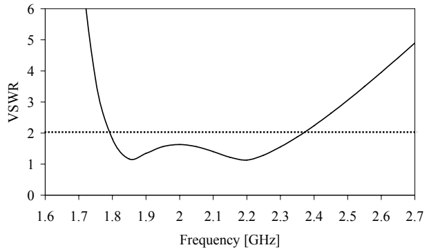
Fig. 2 Simulated VSWR of the proposed patch antenna
