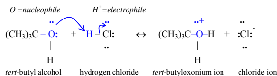
(a) First reaction step. It is a “make-bond” process.
