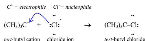
(c) Third reaction step. It is a “make-bond” process.
