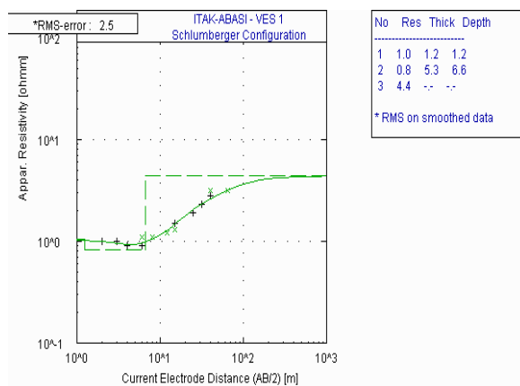
Fig. 1 Geoelectric Sounding Curve Obtained from VES 1
