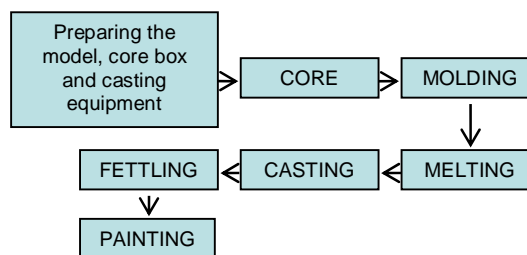
Fig. 1 Manufacturing Line
