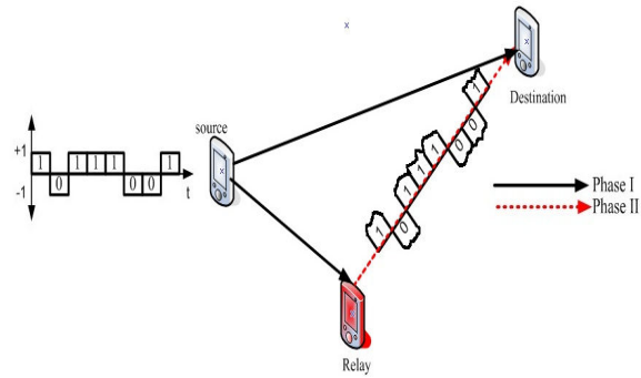
Fig. 2 Amplify and Forward model
