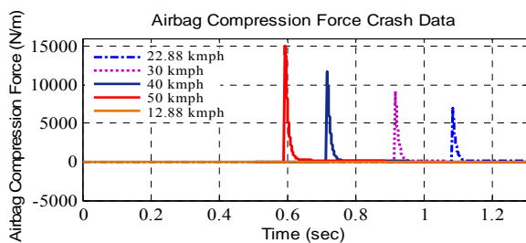
Fig. 14 Airbag compression force during various crashes
