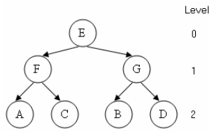
Fig. 2 ADBT of an I^{2^i} image
