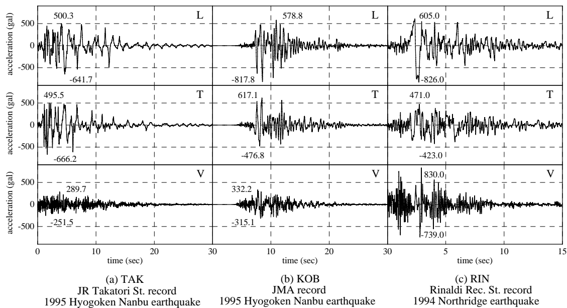
Fig. 5 Input earthquake ground motions
