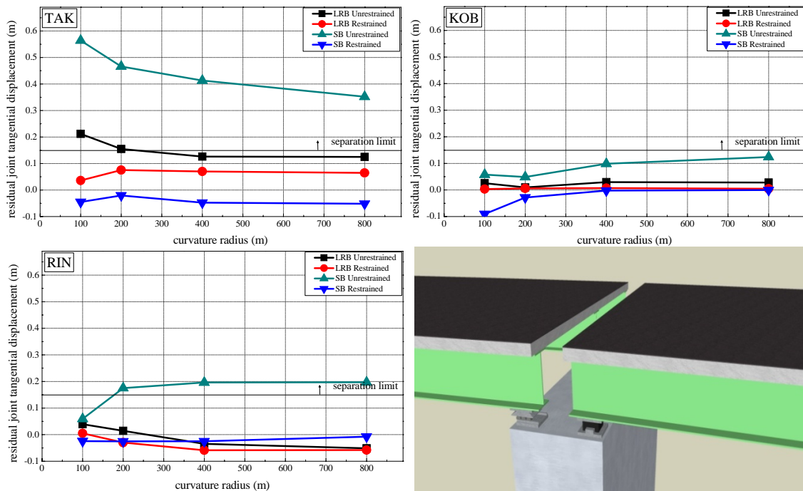
Fig. 7 Curvature effect on tangential joint residual damage
