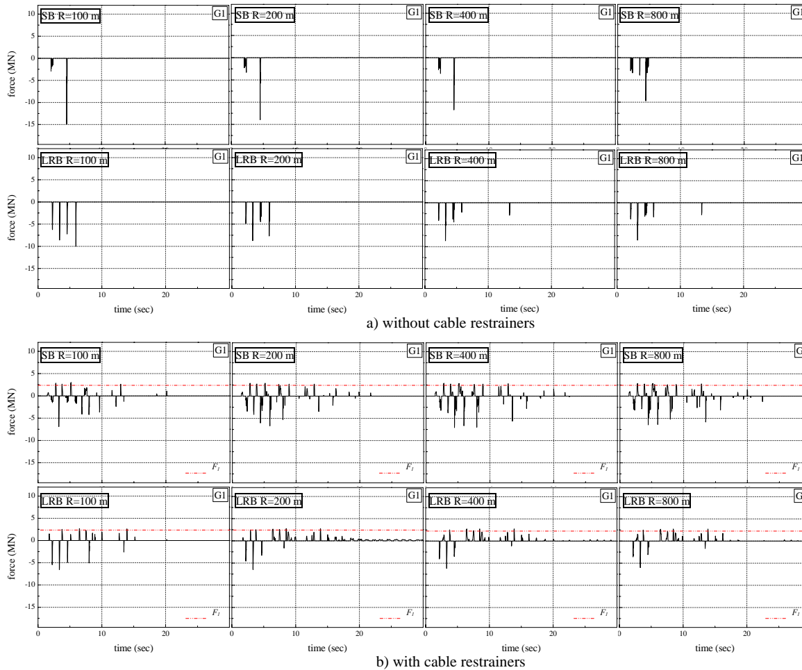
Fig. 8 Maximum Impact forces at expansion joint from TAK
