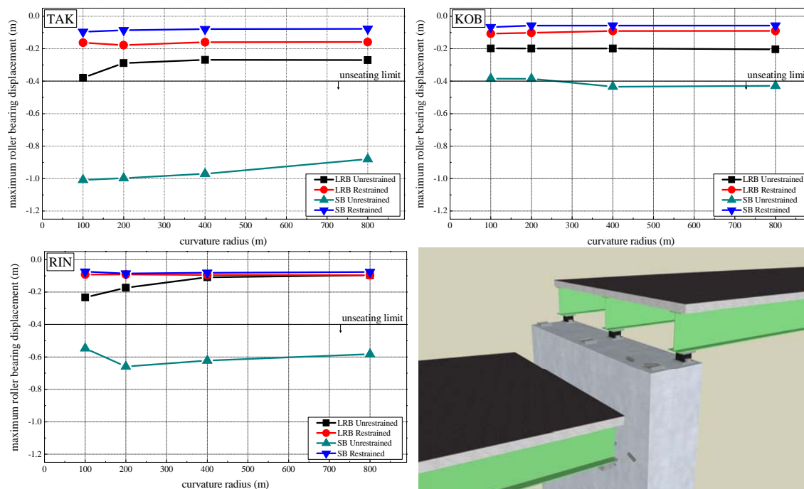
Fig. 6 Curvature effect on deck unseating damage
