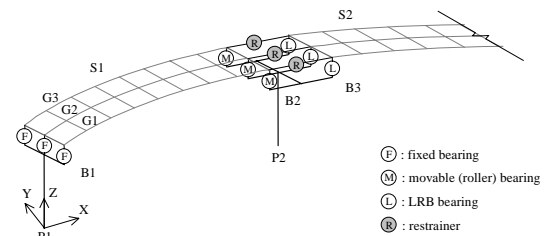
Fig. 2 Detail of curved viaduct finite element model
