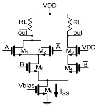
Fig. 1 CML NAND/AND logic schematic
