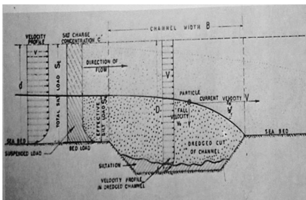
Fig. 12 Diagram to estimate siltation in basin/channel [5]
