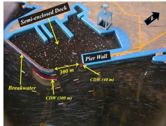
Fig. 8 Locations of CDW near Dock
