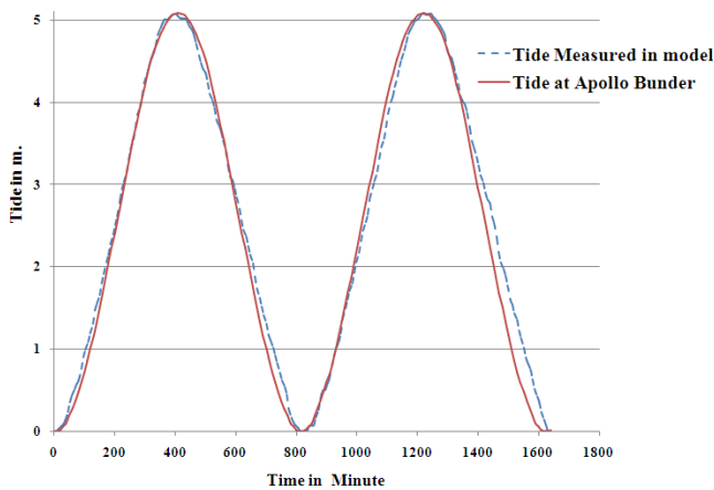
Fig. 5 Comparison of Proto and Model Tide Data
