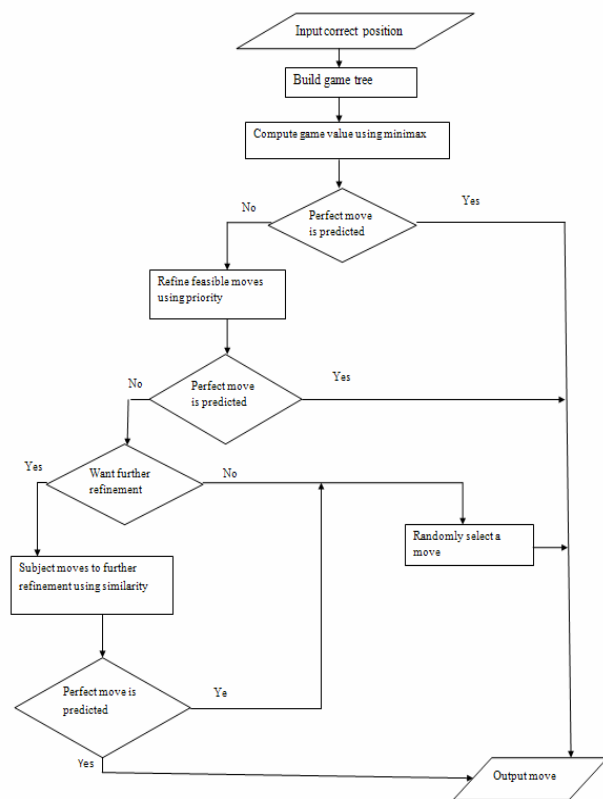
Fig. 5 Flowchart Showing the Refinement Procedure
