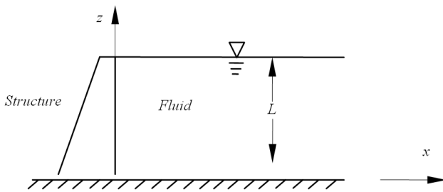
Fig. 1 Fluid-structure system
