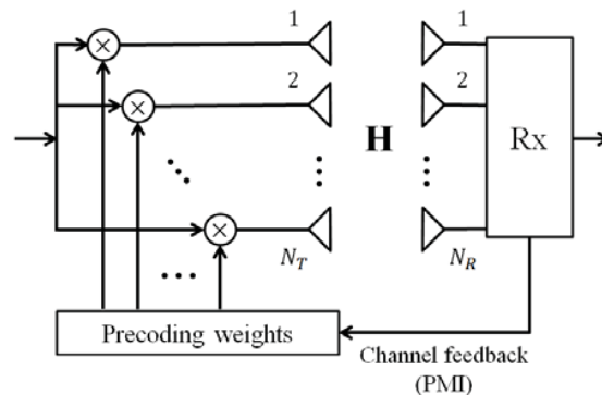
Fig. 1 Closed-loop MIMO transceiver using PMI
