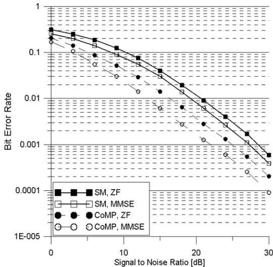
Fig. 4 The BER performance for the four schemes
