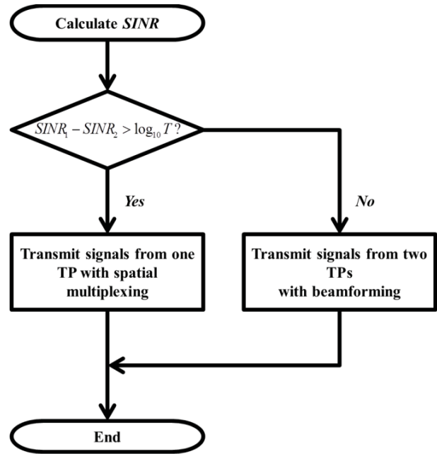
Fig. 3 The block diagram for the proposed scheme
