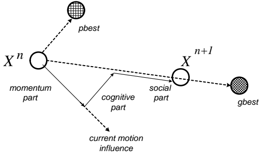
Fig. 4 Position updates of particles in particle swarm optimization technique
